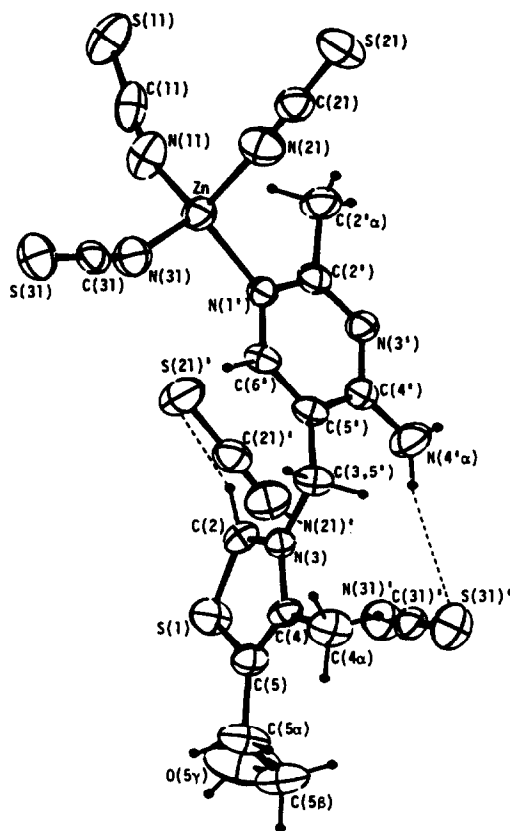
Fig. 25. Crystal structure of \text{Zn}(\text{Th})(\text{SCN})_3 showing an \text{N}(4')\cdots\text{S}(31')\text{—C}(31')\text{—N}(31')\cdots thiazolium ring interaction (“one-point” anion bridge). Reproduced by permission from ref. 57.
