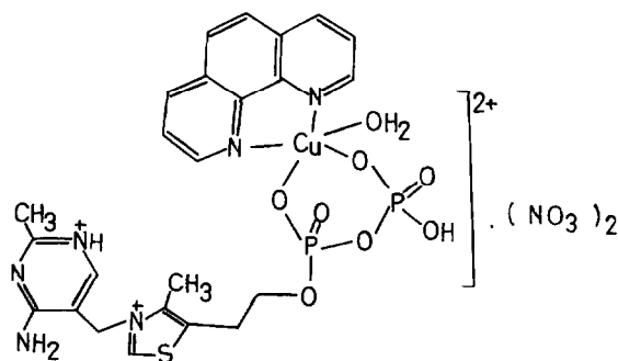
Fig. 10. Structure of the complex [\text{TPP}-\text{Cu}^{2+}-\text{phen}](\text{NO}_3)_2 .
