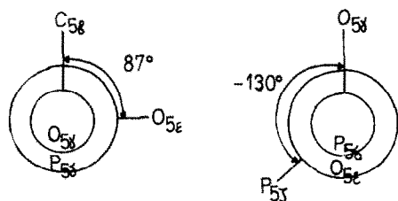
Fig. 16. Newman projections along the O(5\gamma) – P(5\delta) and P(5\delta) – O(5\epsilon) bonds of the complex [TPP \cdot Cu^{2+} - phen] .
