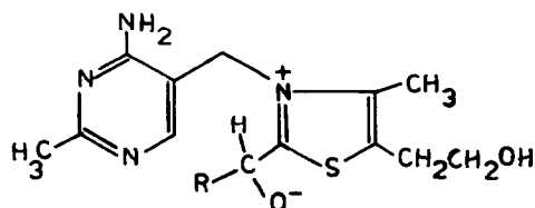
Fig. 2. Structure of the “active aldehyde” derivative.
