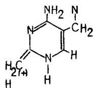
Fig. 12. Hyperconjugate resonance structure of pyrimidine of thiamine.
