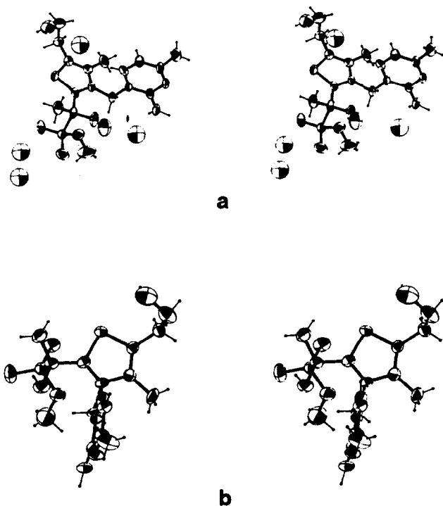
Fig. 21. Crystal structure of PLT·HCl·3H 2 O. Reproduced by permission from ref. 64.
